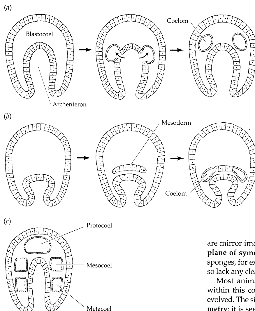
Figure 1.11 Coelom formation by entero-coely (frontal sections). (a) Archenteric pouching. (b) Proliferation and subsequent hollowing of a plate of mesoderm from the archenteron. (c) The typical tripartite arrangement of coeloms in a deuterostome embryo. (From Brusca and Brusca 1990.)
