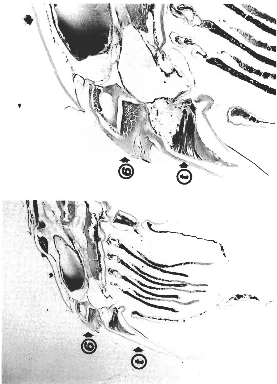
FIG. 13. Paranthura elegans (Anthuridea). Median saggital section through pleon showing fusion of pleomeres 5 and 6, and fusion of pleomere 6 with telson. Despite fluting, a continuous cuticular covering connects these somites and no articular membranes are present. Also note large opercular first pleopods. Arrows indicate pleomere and telson.
