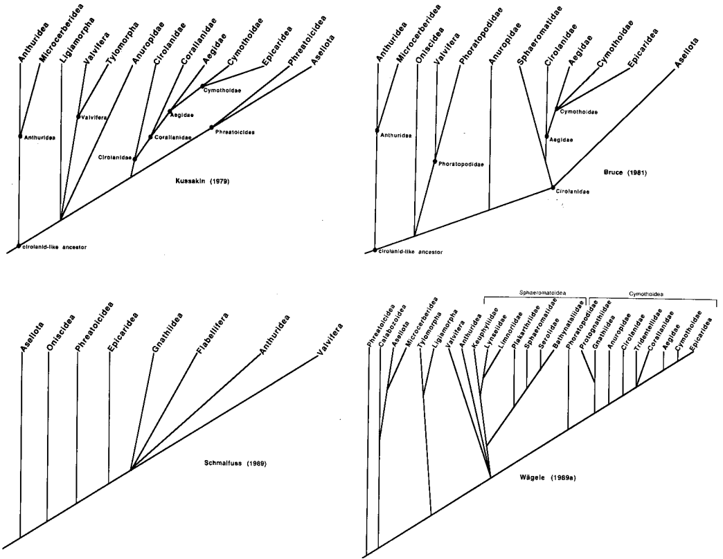
FIG. 4. Some evolutionary trees from previous studies, by Kussakin (1979), Bruce (1981), Schmalzfuss (1989), and Wägele (1989a).
