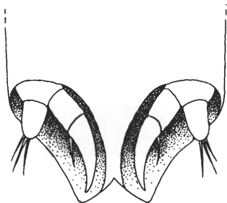
FIG. 11. Keuphylia (Keuphylidae). Ventral view of pleotelson showing arrangement of uropods in ventral pocket.
