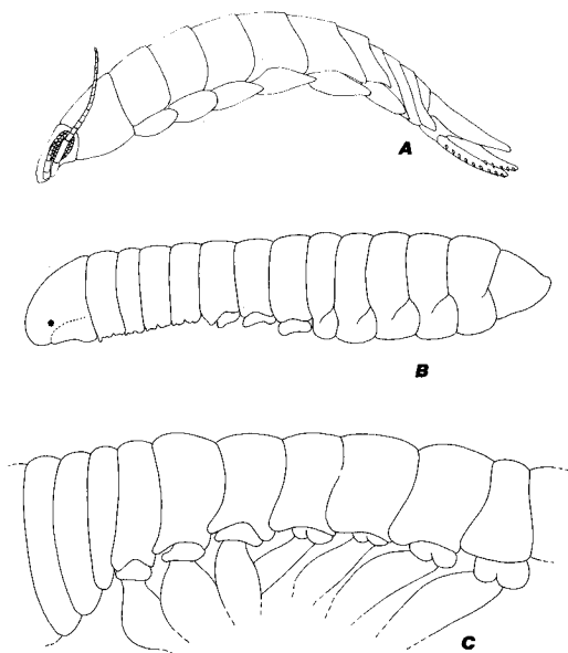
FIG. 9. Lateral views of a flabelliferan and two phreatoicidans, illustrating development of the pereopodal coxae. A, Rocinela propodialis (type, USNM 29248). B, Phreatoicopsis terricola (USNM 78431). C, Phreatoicus australis (USNM 59116; anterior is to the right).
